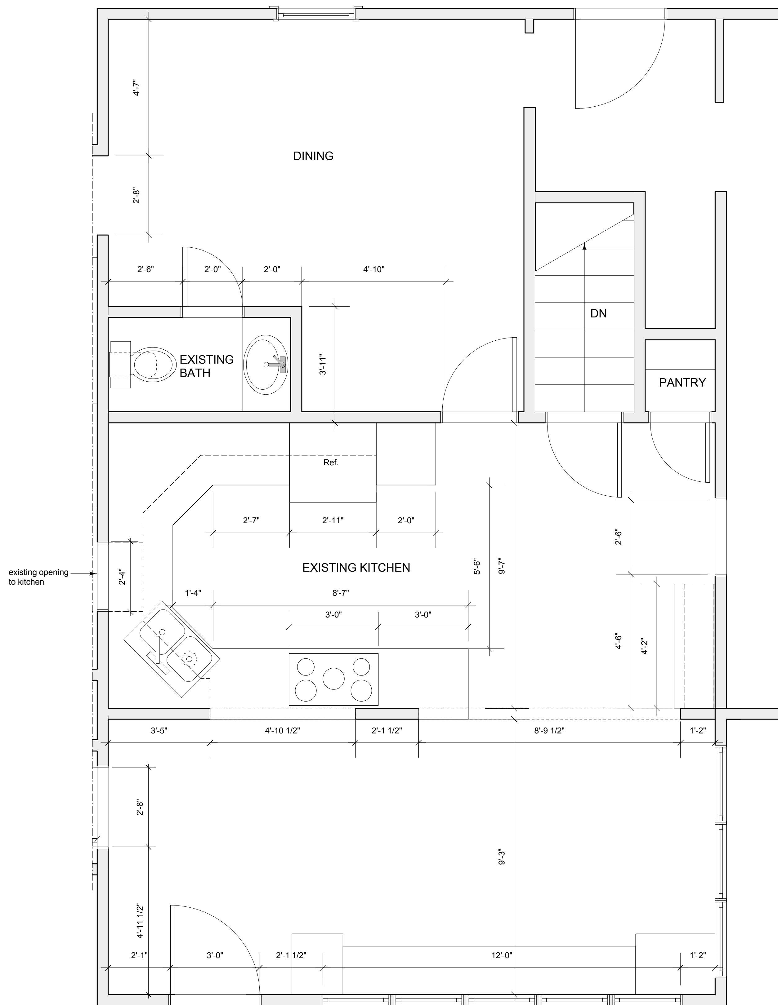
1 Kitchen - Existing Plan A2 Scale: 1/2" = 1'-0"
